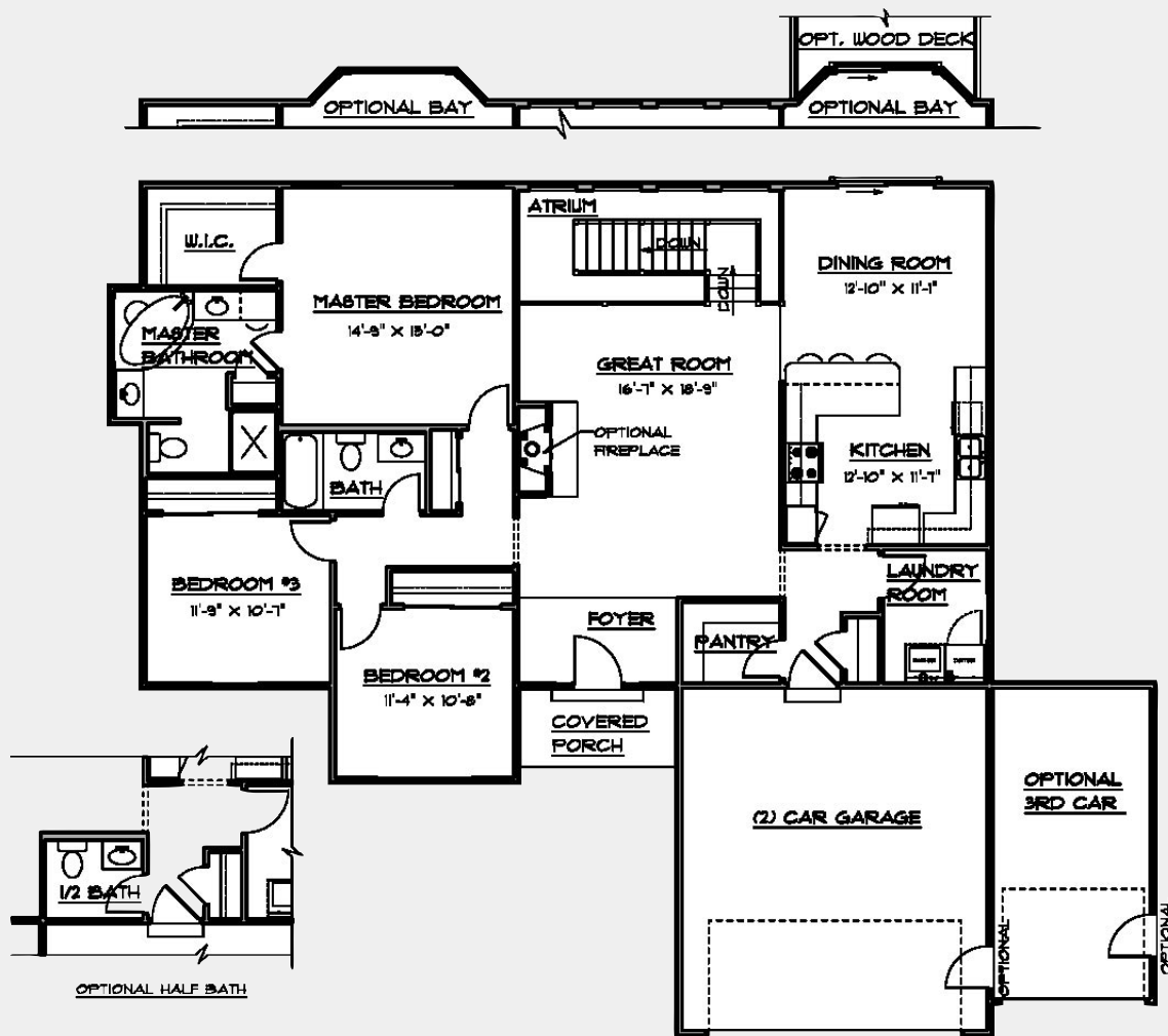
FIRST FLOOR
